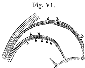
Fig. VI. Section of two septa of Operculina through the median plane, showing the secondary pores, b, b, b , in addition to the principal orifices, a, a , at the inner margin of the spire.
